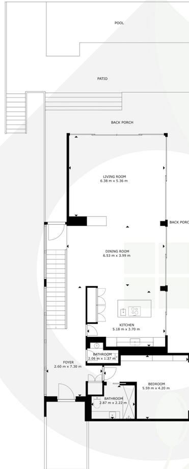
MAIN FLOOR
