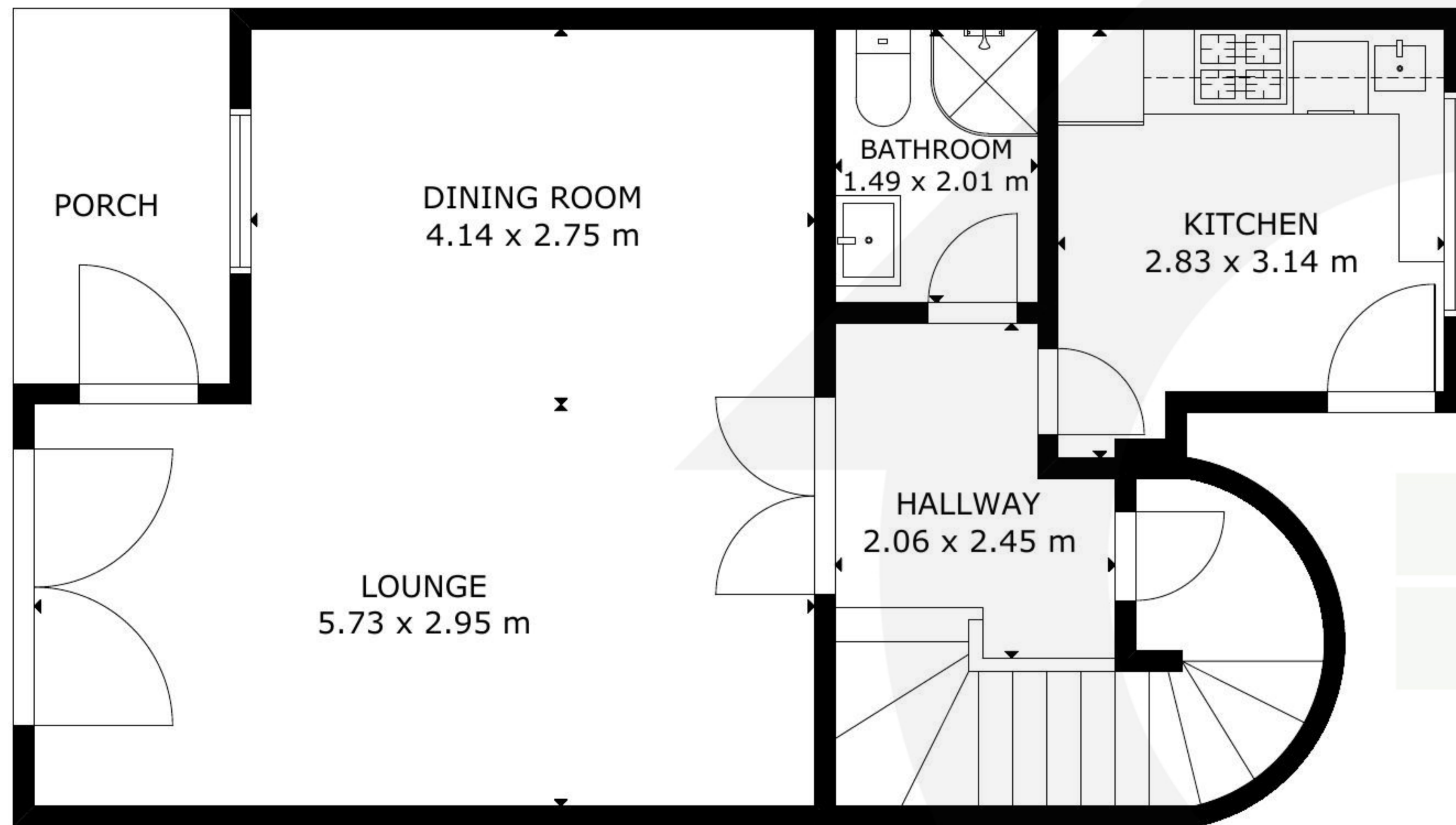
GROUND FLOOR
