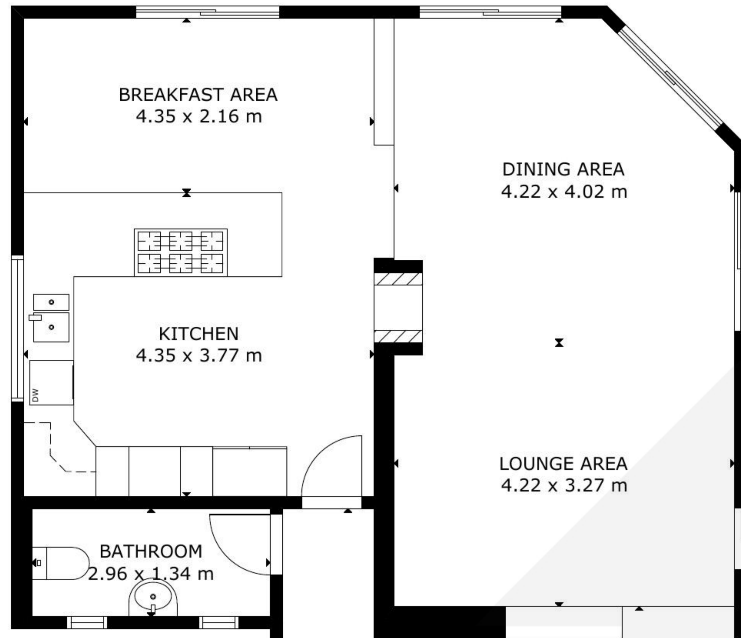
GROUND FLOOR
