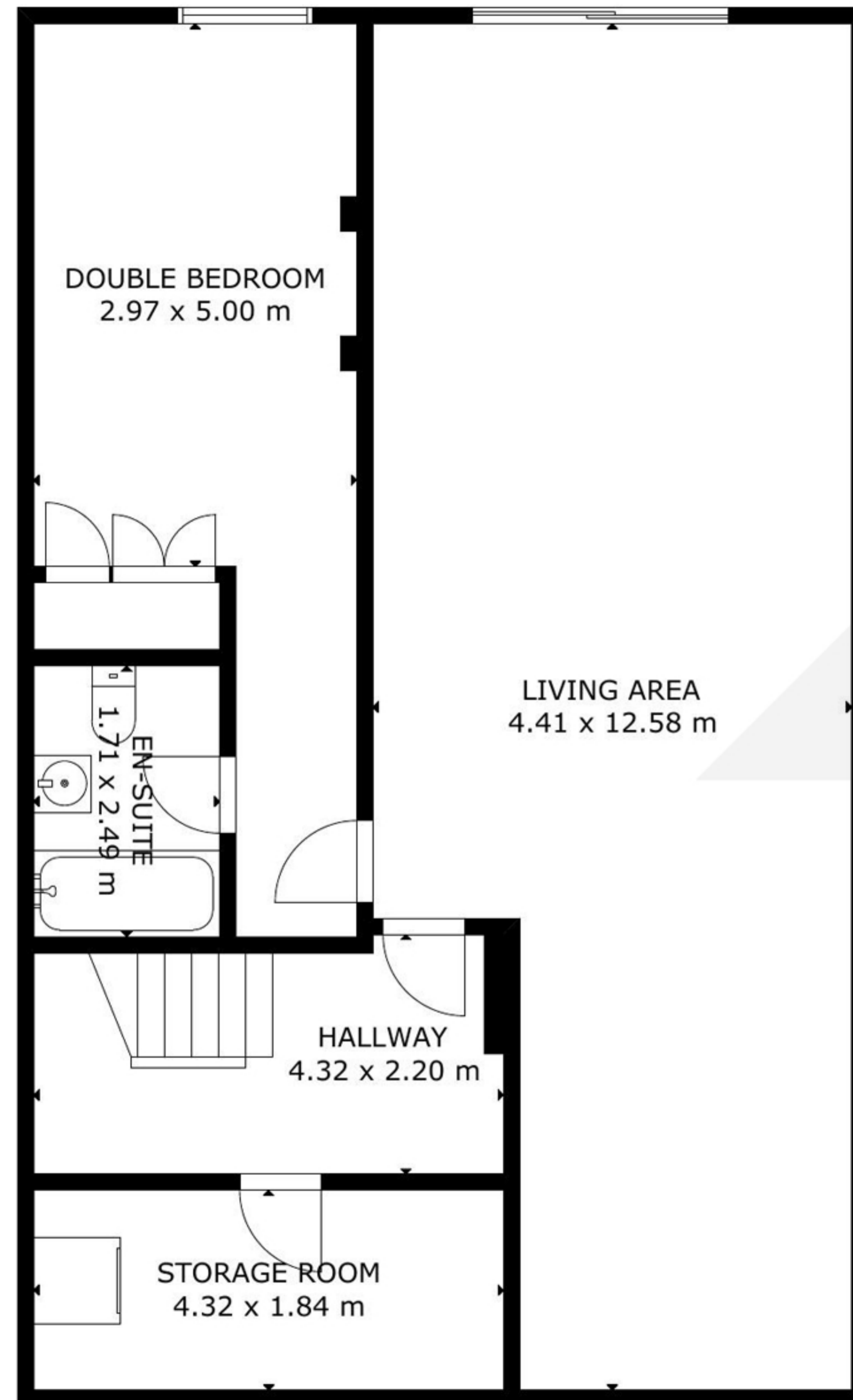
BASEMENT
