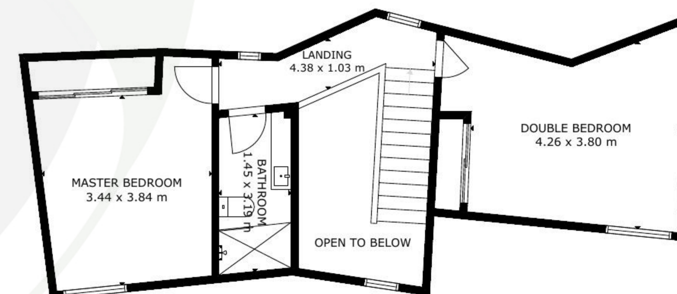
SECOND FLOOR
