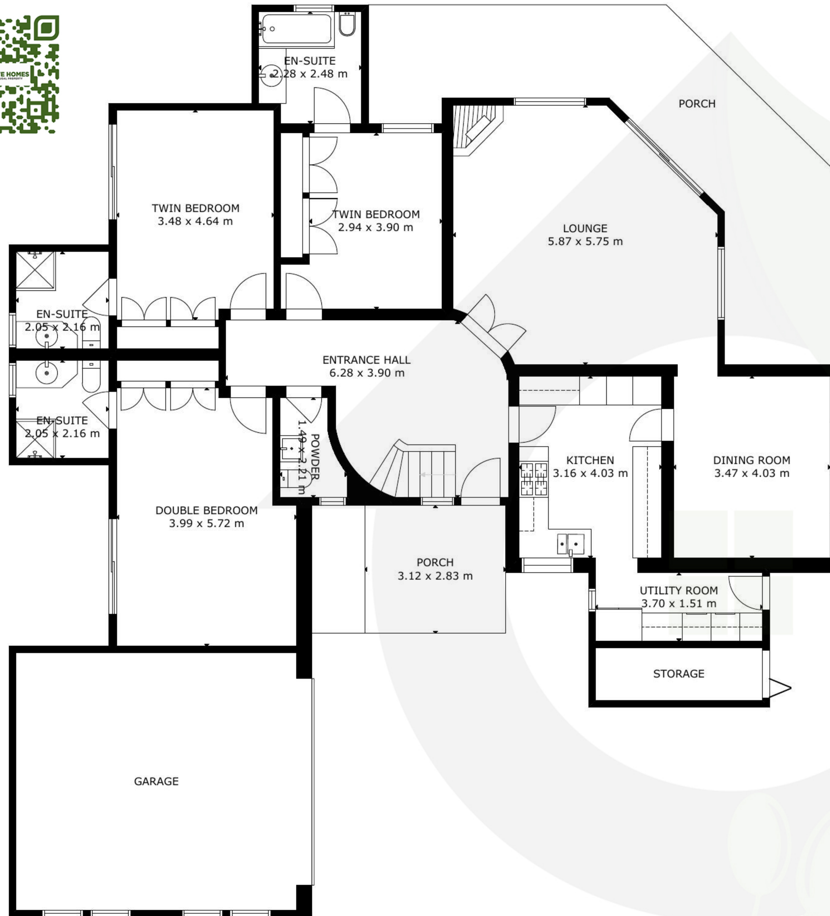
GROUND FLOOR
