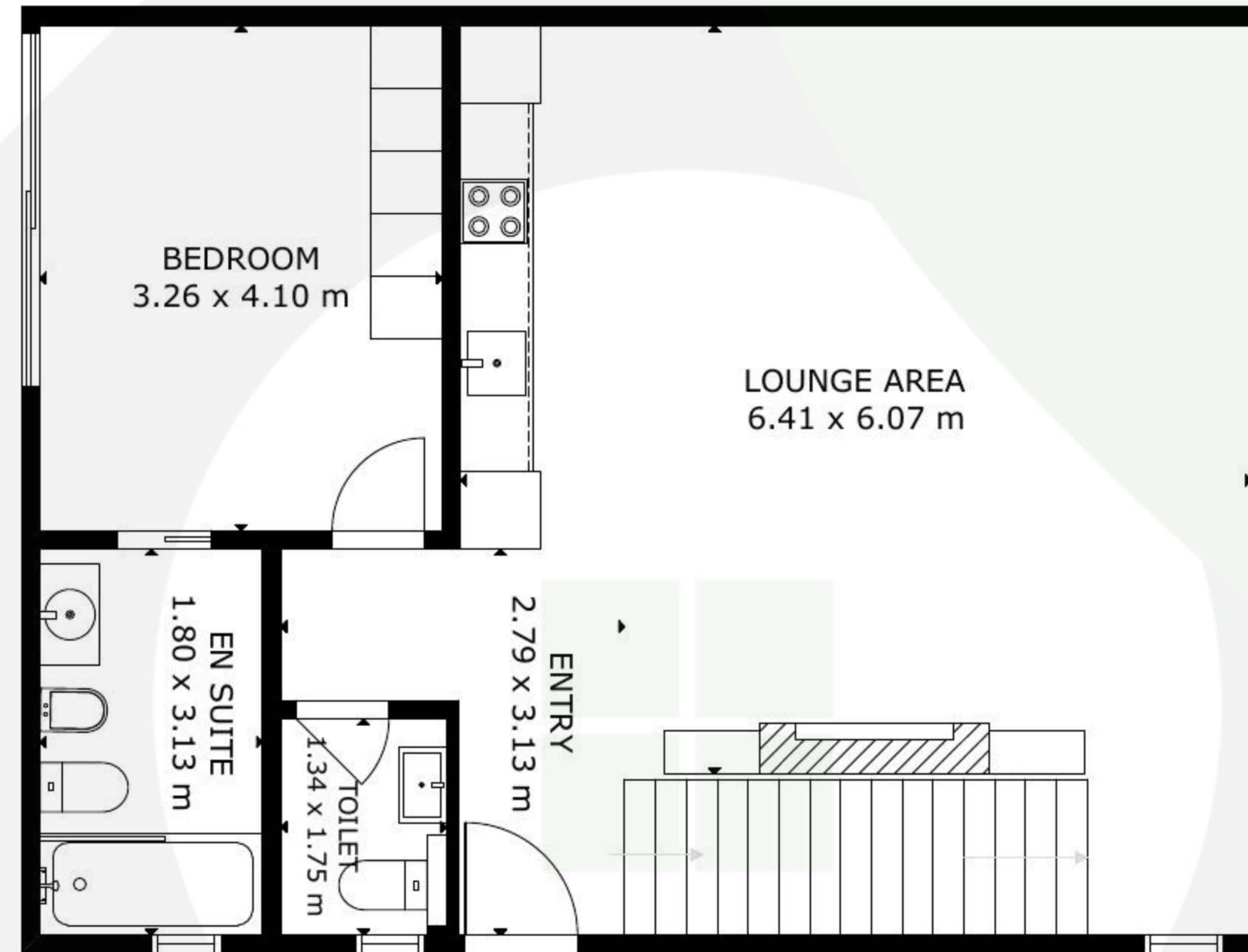
GROUND FLOOR
