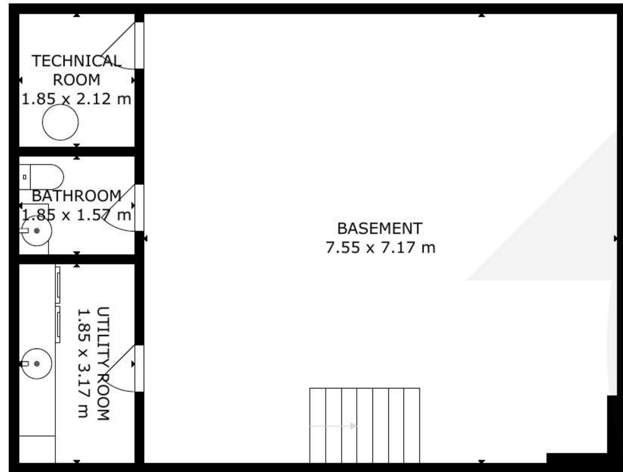
BASEMENT
